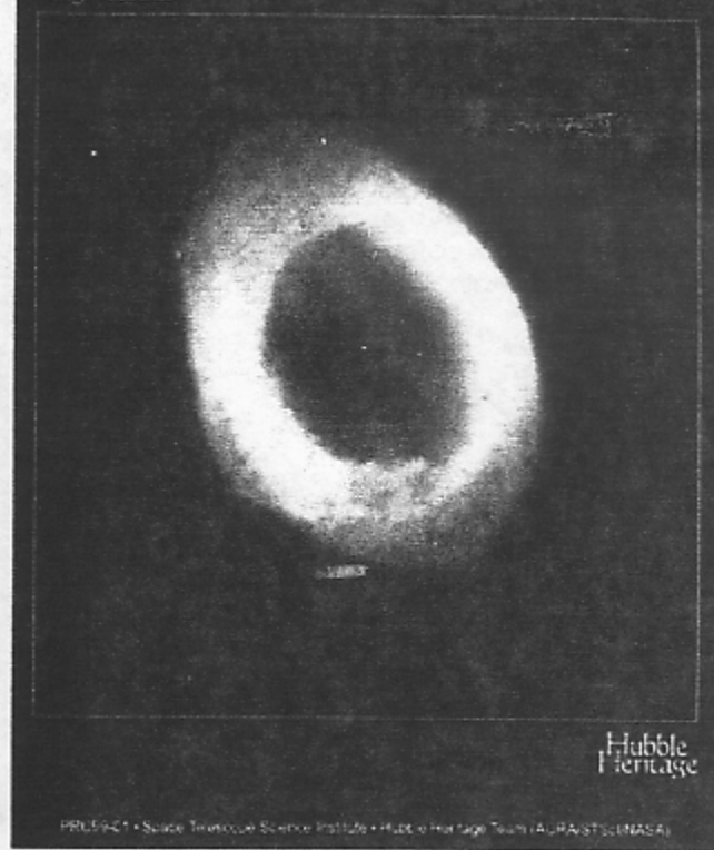
Ring Nebula
